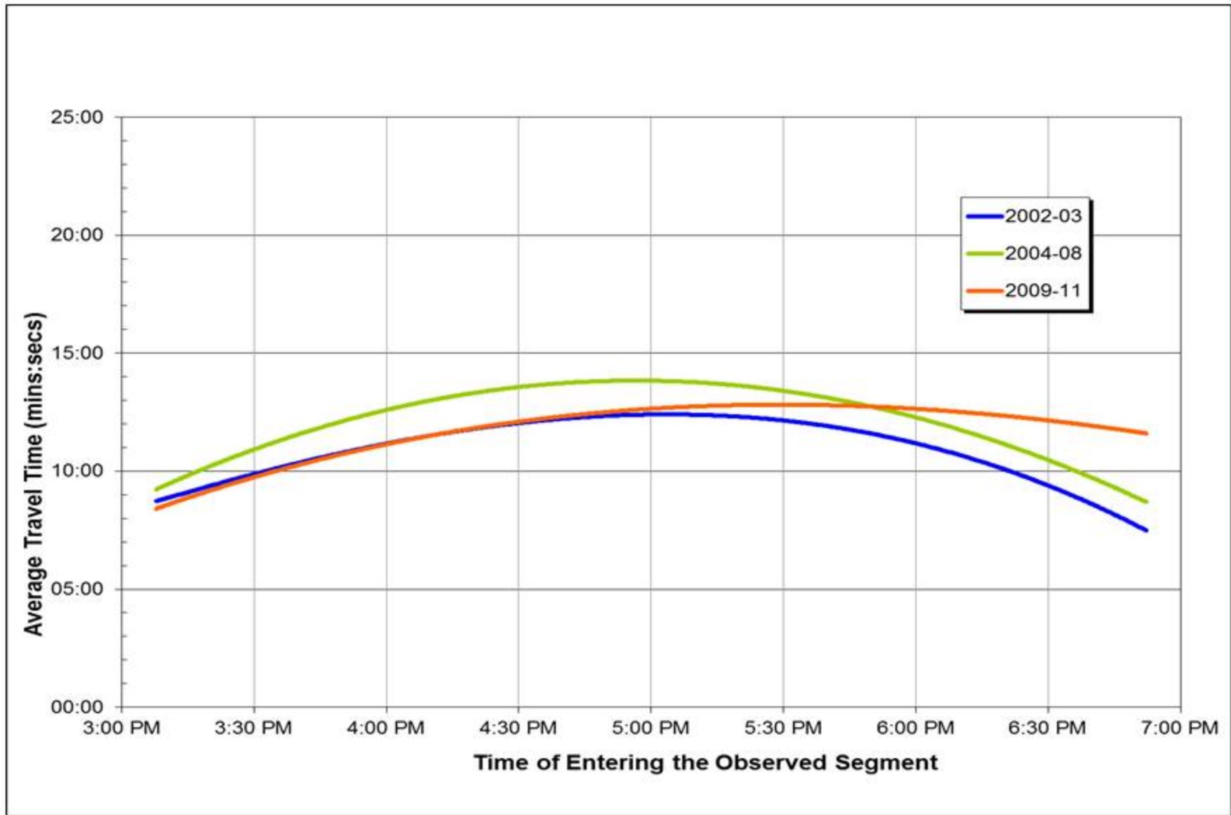
FIGURE 9 Southeast Expressway Travel Times: Southbound General-Purpose Lanes, PM Peak Period, 2002-11
