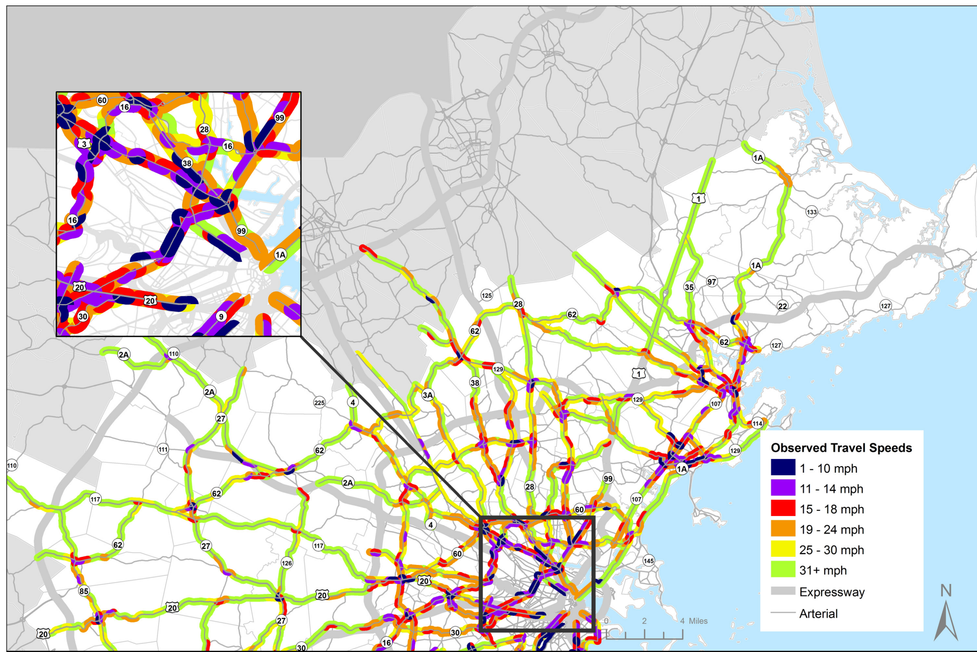
BOSTON REGION MPO Travel Speeds for Arterials: Northern Half of MPO Area, AM Peak Period, 2001-08 Congestion Management Process
