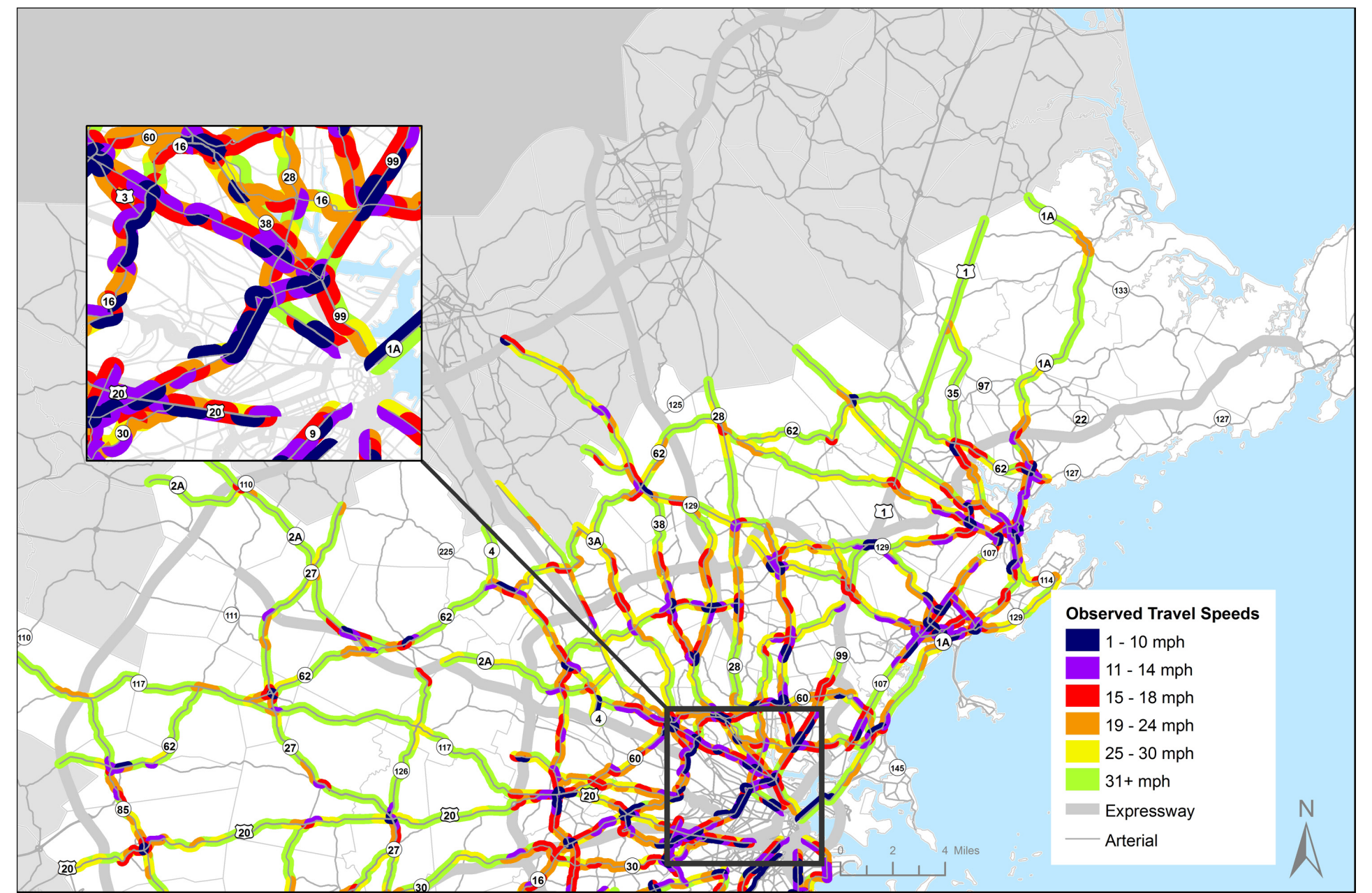
BOSTON REGION MPO Travel Speeds for Arterials: Northern Half of MPO Area, PM Peak Period, 2001-08 Congestion Management Process
