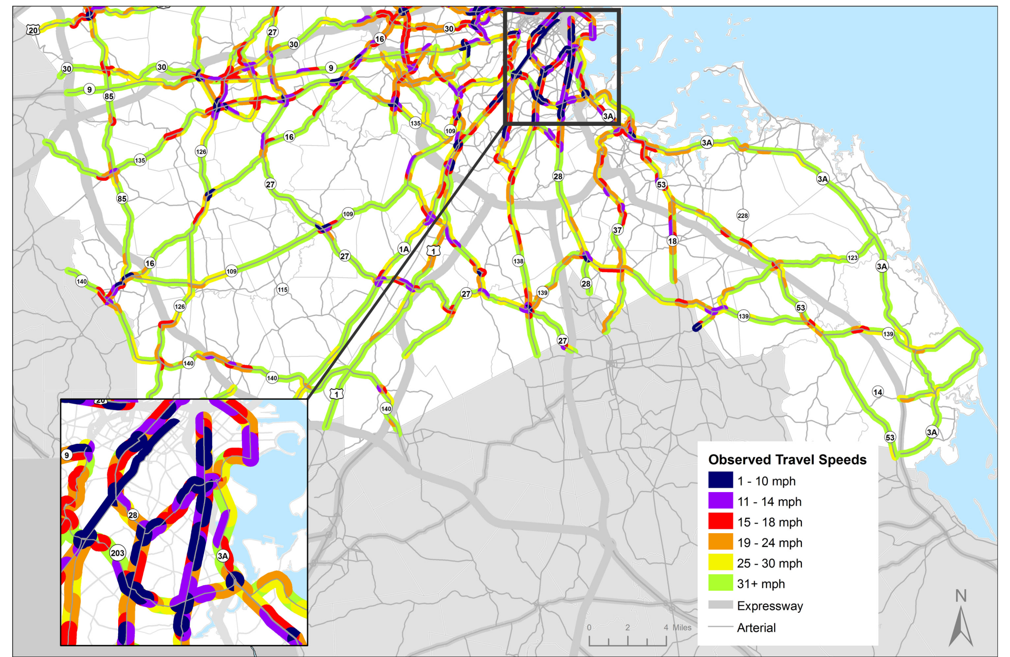
BOSTON REGION MPO Travel Speeds for Arterials: Southern Half of MPO Area, PM Peak Period, 2001-08 Congestion Management Process
